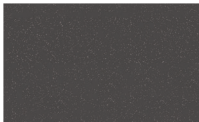
Graphite (Metallic)
